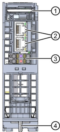
Figure 2-4 View of the CPU 1511-1 PN (without front panel) – front
