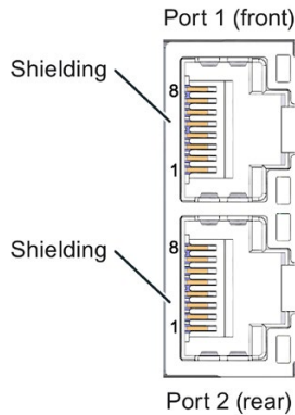
Figure 3-2 PROFINET ports
